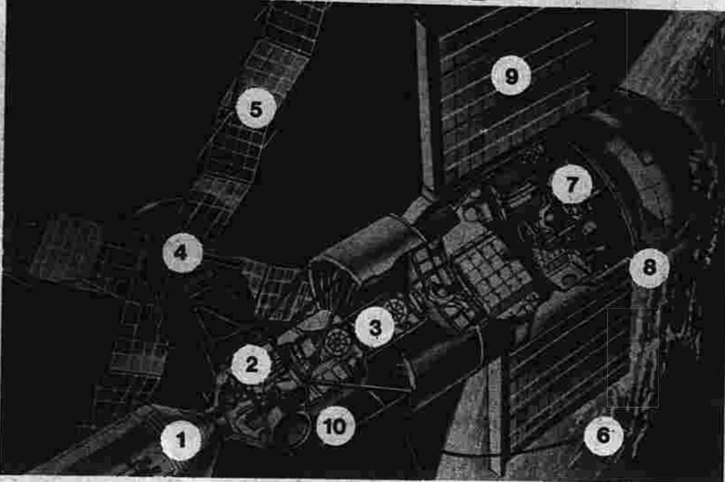
The parts of Skylab: 1. Apollo command and service module, 2. Module dock, 3. Environmental and electrical control center, 4. Telescope mount for solar experiments, 5. Solar arrays (or wings) that help provide electrical power, 6. Workshop, 7. Crew quarters, 8. Protective shield, 9. Solar arrays that help provide electrical power for the workshop, 10. Earth resource experiments.
